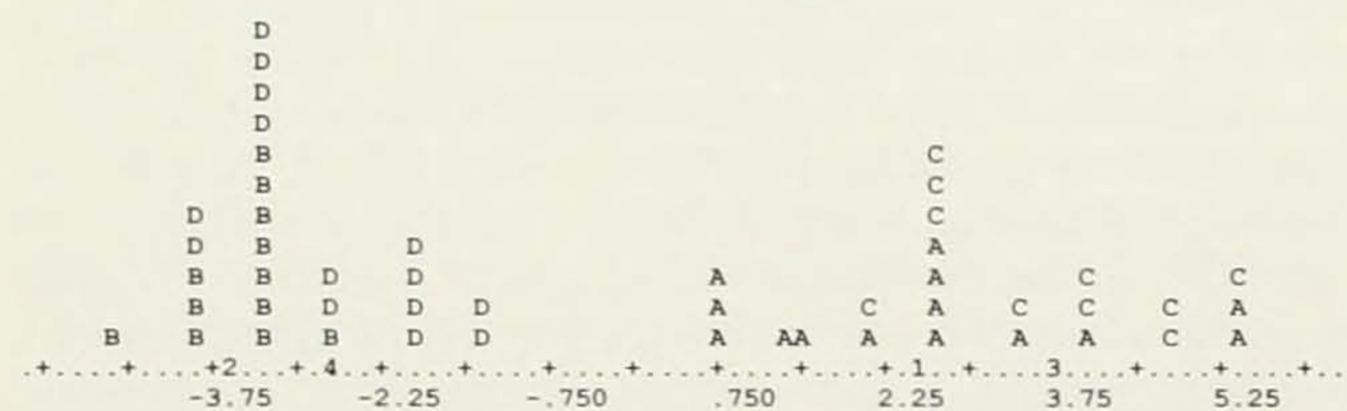
Figure 5. Histogram of the canonical variable resulting from a stepwise discriminant analysis of the core sample of 10 specimens of Cistothorus palustris plesius/pulverius and all Marsh Wren specimens from the San Joaquin delta. The discriminant function was based on the core specimens, and was used to classify the remaining specimens. Underpart color, rump/scapular color, wing length, back pattern, and crown pattern, in decreasing order of importance, are the informative variables. C, core specimens of plesius/pulverius ; D, core specimens of aestuarinus ; A, inferred specimens of plesius/pulverius ; B, inferred specimens of aestuarinus .
