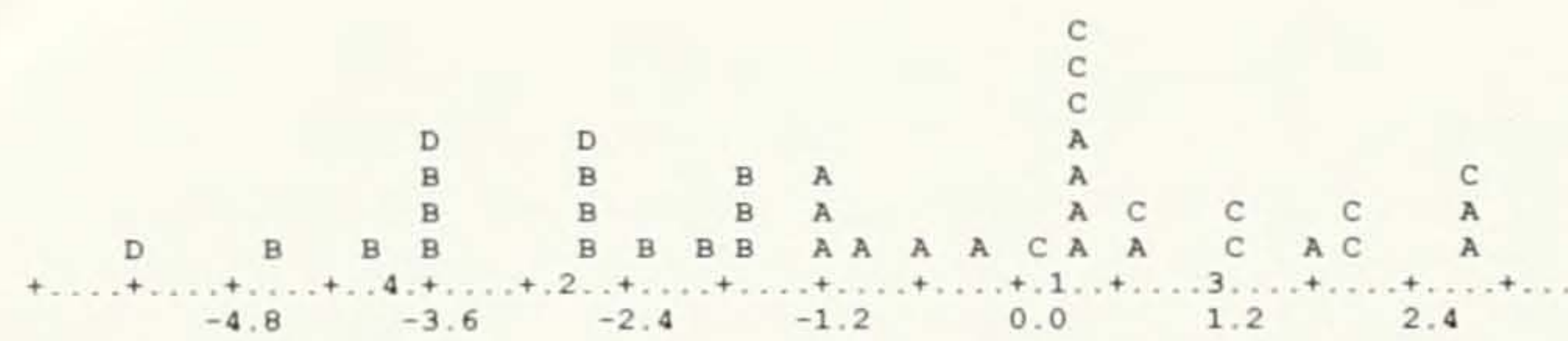
Figure 4. Histogram of the canonical variable resulting from a stepwise discriminant analysis of the core sample of 10 specimens of Cistothorus palustris plesius/pulverius and all Marsh Wren specimens from the Imperial and lower Colorado River valleys. The discriminant function was based on the core specimens, and was used to classify the remaining specimens. Rump/scapular color, underpart color, wing length, and crown pattern, in decreasing order of importance, are the informative variables. C, core specimens of plesius/pulverius ; D, core specimens of deserticola ; A, inferred specimens of plesius/pulverius ; B, inferred specimens of deserticola .
