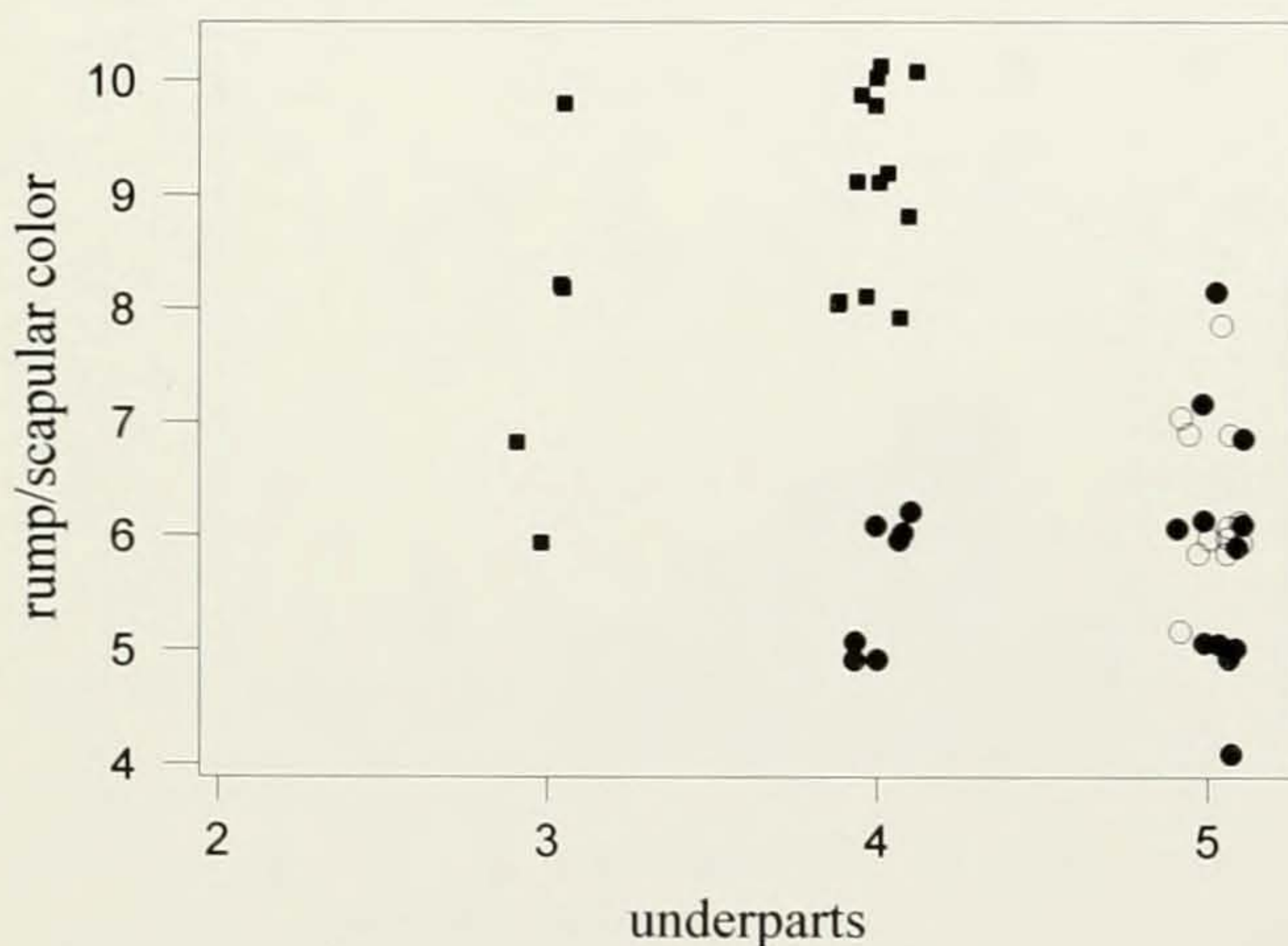
Figure 18. Scatterplot for Cistothorus palustris aestuarinus and coastal southern California Marsh Wrens of the pair of variables in which they differ most, rump/scapular color and underparts. ●, core (September) specimens from the San Joaquin Delta ( aestuarinus ); ○, additional (October) specimens from the San Joaquin Delta (inferred aestuarinus ); ■, specimens of the breeding population of coastal southern California.
