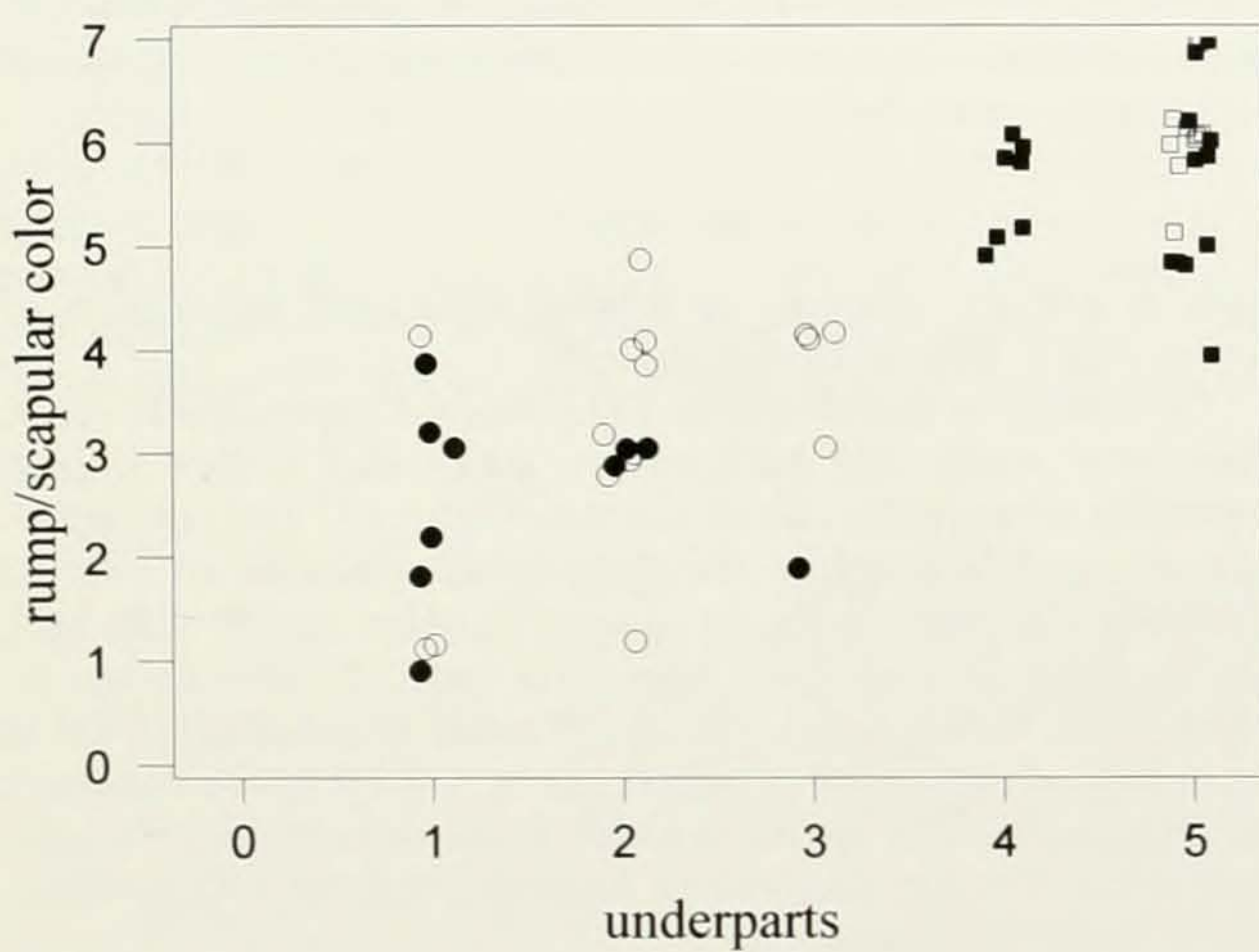
Figure 10. Scatterplot for Cistothorus palustris plesius/pulverius and C. p. aestuarinus of the two variables in which they differ most, underpart color and rump/scapular color. ●, core-sample specimens of plesius/pulverius ; ○, inferred specimens of plesius/pulverius ; ■, core-sample (September) specimens from the San Joaquin Delta ( aestuarinus ); □, additional (October) specimens from the San Joaquin Delta (inferred aestuarinus ).
