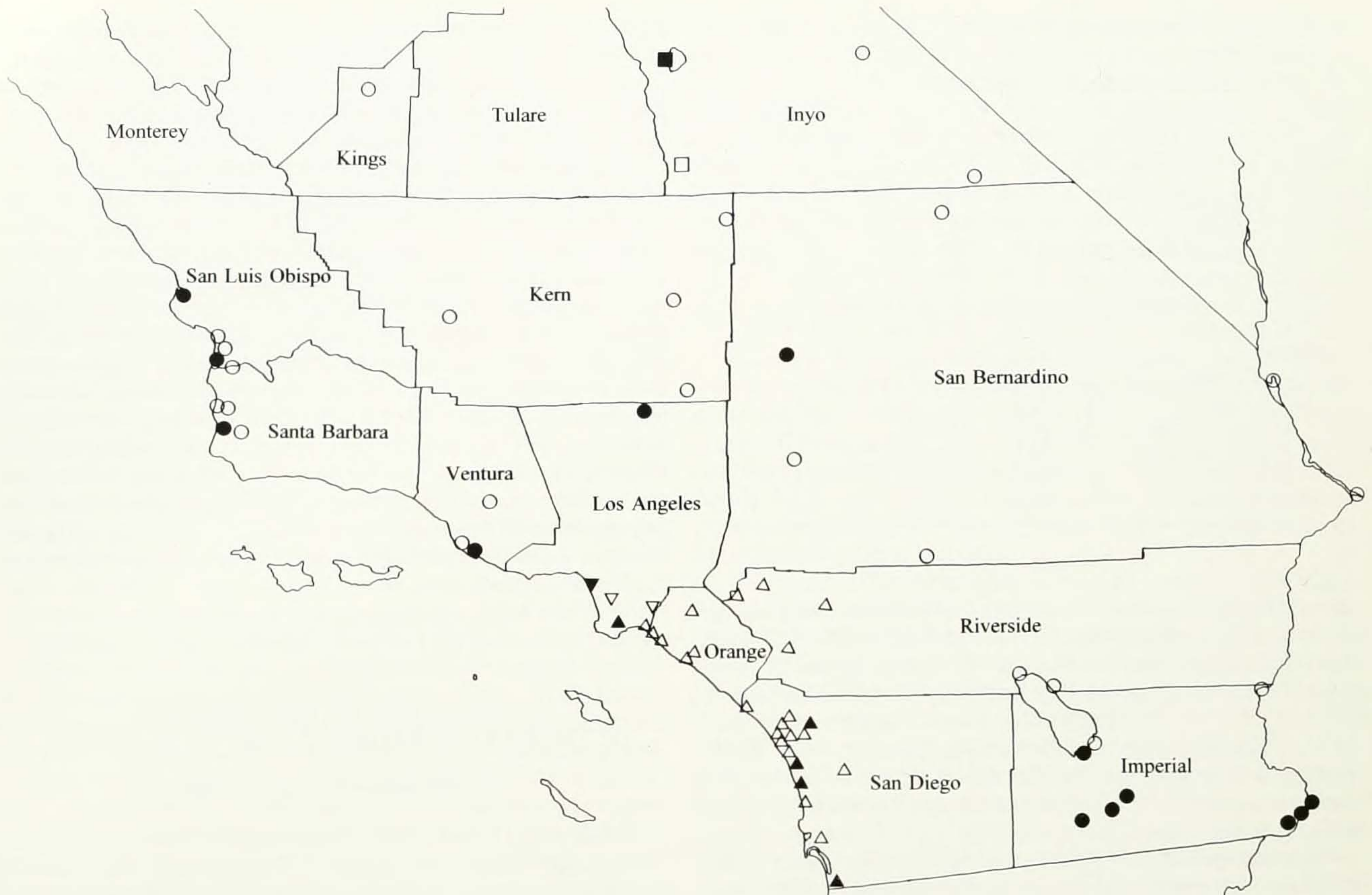
Figure 22. Distribution of the Marsh Wren as a breeding species in southern California. Squares, Cistothorus palustris pulverius ; circles, C. p. aestuarinus (including deserticola ); upright triangles, recent sites for C. p. clarkae ; inverted triangles, former sites for C. p. clarkae . Filled symbols, specimens examined; open symbols, other sites where the Marsh Wren is known to have bred or summers regularly (subspecies allocation inferred at these sites). These sites are based on published literature, personal observation, personal communication from many field ornithologists, and the egg collections of the Western Foundation for Vertebrate Zoology, Camarillo, and the San Bernardino County Museum, Redlands.
