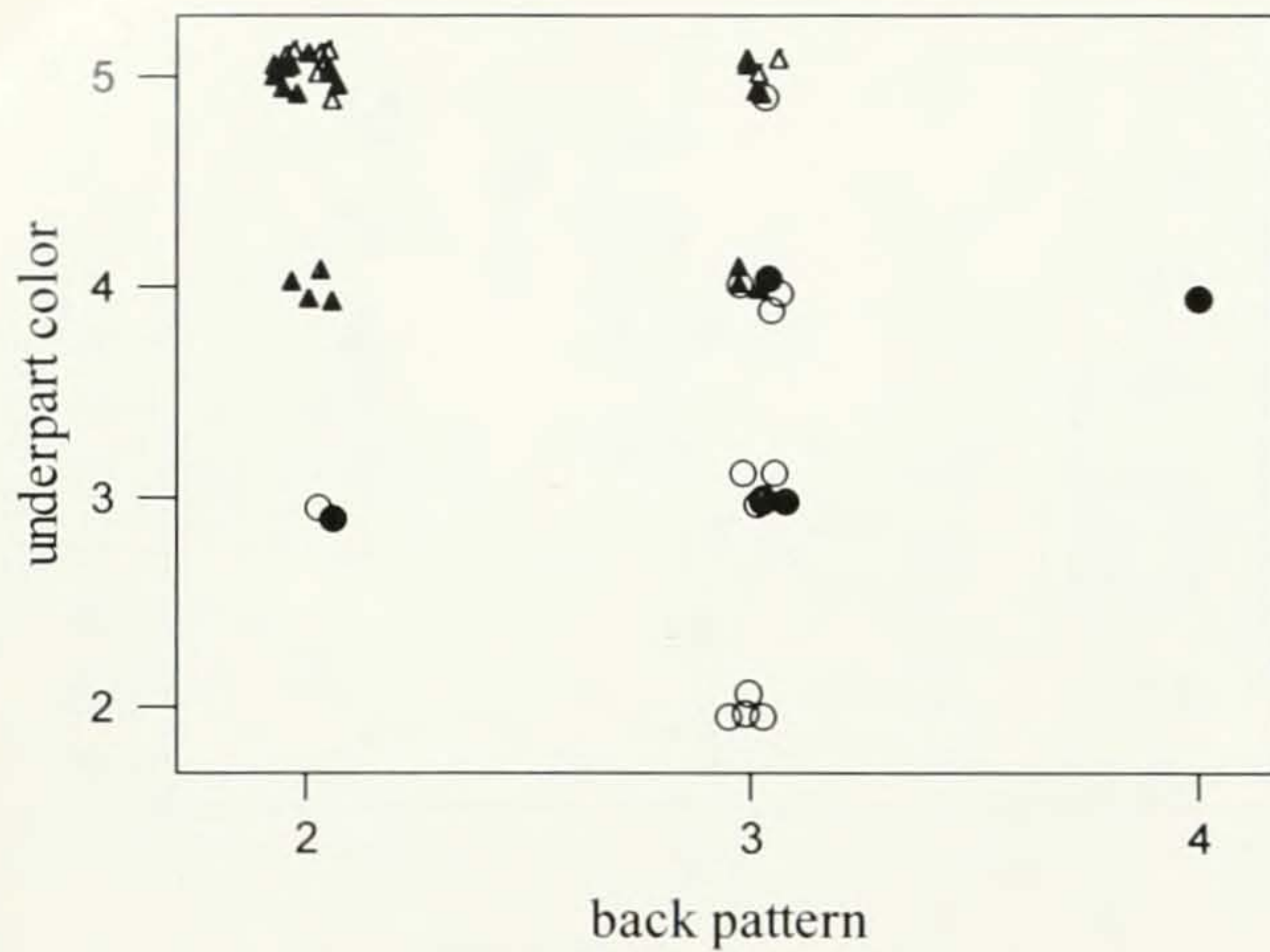
Figure 17. Scatterplot for Cistothorus palustris aestuarinus and C. p. deserticola of the only two variables in which they differ significantly, underpart color and back pattern. ▲, core (September) specimens from the San Joaquin Delta ( aestuarinus ); △, additional (October) specimens from the San Joaquin Delta (inferred aestuarinus ); ●, core (August/September) specimens of the breeding population of the Colorado Desert ( deserticola ); ○, additional October–February specimens from the Colorado Desert inferred as deserticola (see Figure 4).
